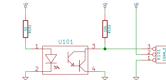
OPTICAL_SENSOR_WITH_PHOTOTRANSISTOR
